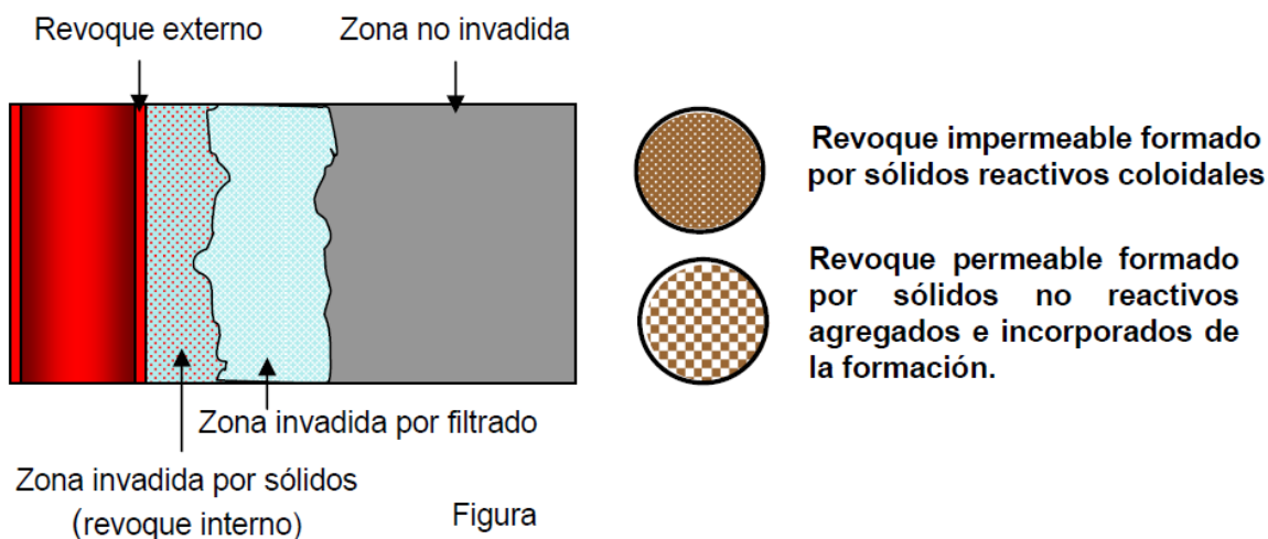
Figura 23 - Revoque (Prieto, 2007) [13]
