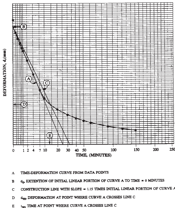
FIG. 3 Time-Deformation Curve From Square Root of Time Method
