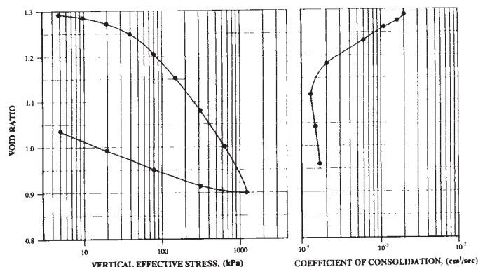
FIG. 5 Example of Consolidation Test Summary Plots
