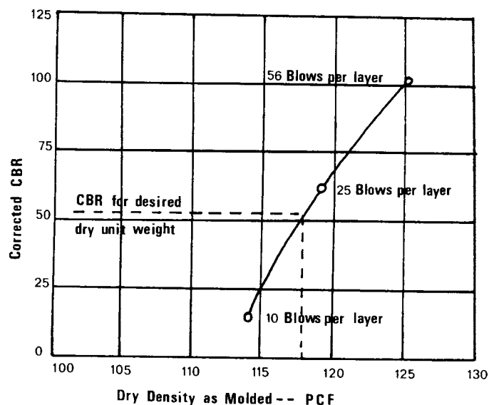
FIG. 3 Dry Density Versus CBR
