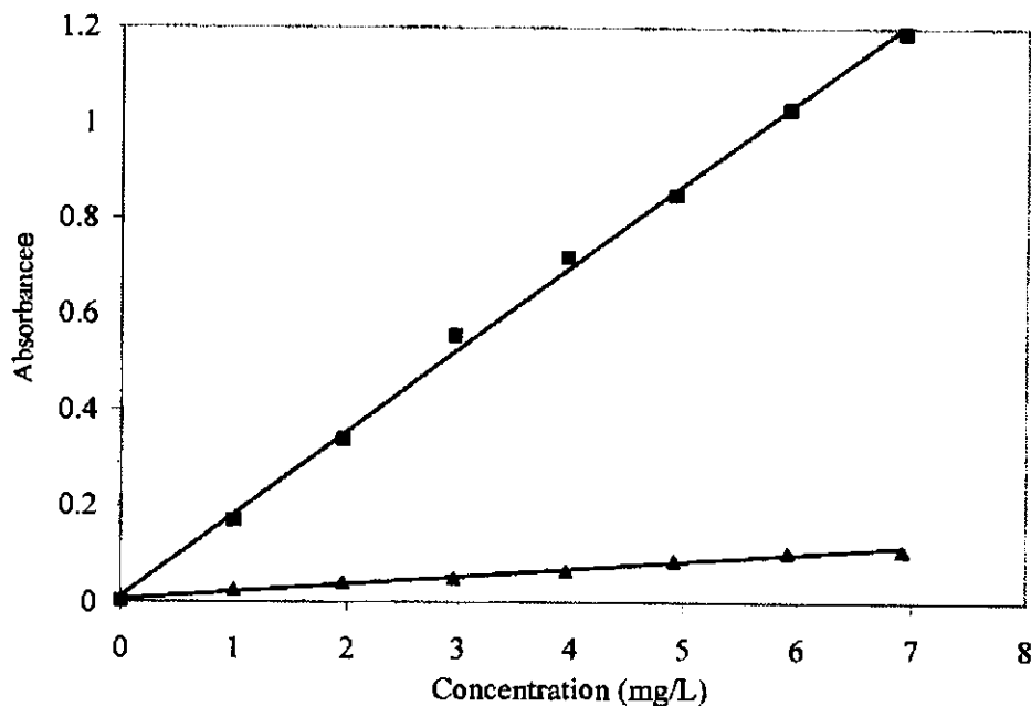
Figure 6. Calibration curves for Neutral red obtained with conventional spectrometer (■) and the proposed WebCam instrument (▲).
