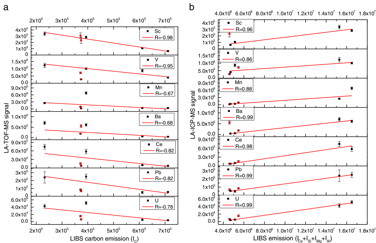
Fig. 5. Correlation analysis between the emission and mass spectra among different coal samples (a) relationship between each trace element mass signal and carbon emission signal ( I_c ); and (b) relationship between each trace element mass signal and total minor elements emission signal ( I_{Ca} + I_{Si} + I_{Mg} + I_{Al} ). Black points indicate the calibration samples and the red ones indicate the validation samples. (For interpretation of the references to color in this figure legend, the reader is referred to the web version of this article.)
