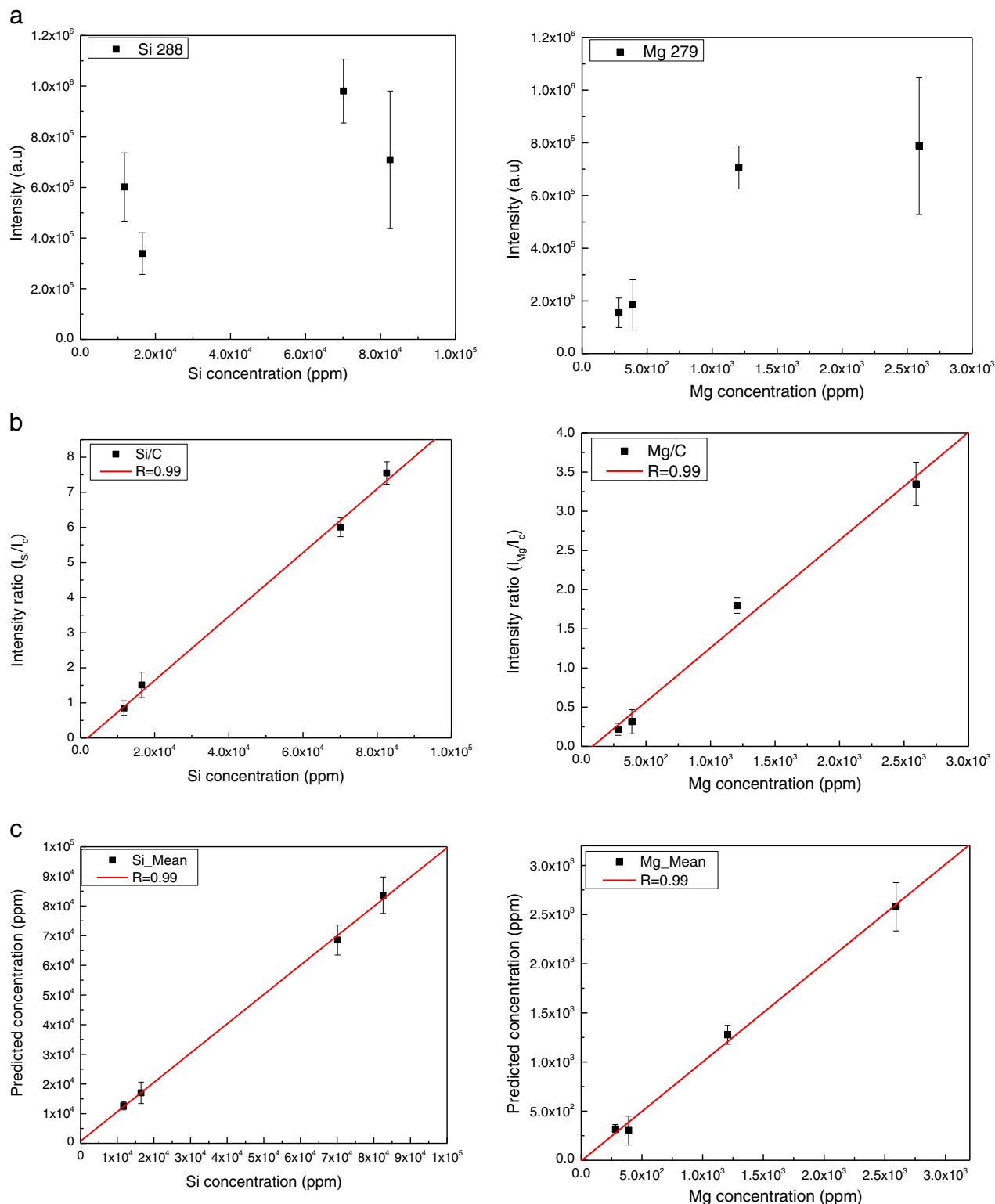
Fig. 3. Comparison of (a) univariate calibration, (b) internal calibration with carbon and (c) multivariable calibration (PLSR) by LIBS for Si and Mg.
