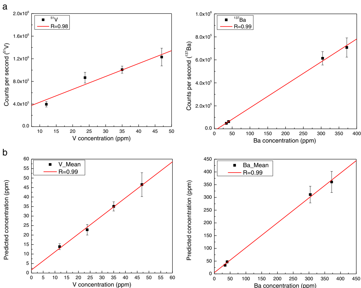
Fig. 4. Comparison of (a) univariate calibration and (b) multivariable calibration (PLSR) by LA-ICP-TOF-MS for V and Ba.
